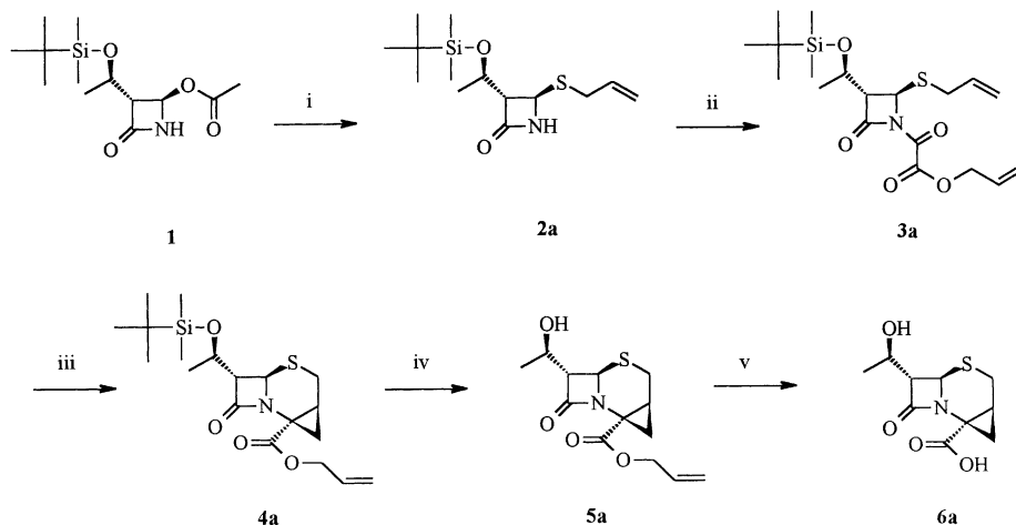
Scheme 1. Reagents: (i) allyl mercaptan, NaH, EtOH, (0°C/2 h, rt/18 h); (ii) allyl chloro-oxalate, Et 3 N, CH 2 Cl 2 (–20°C/1 h); (iii) P(OEt) 3 , xylene (reflux/9 h); (iv) ( i -Pr) 2 EtN·3HF, AcOEt (50°C/10 h); (v) Pd(PPh 3 ) 4 , PPh 3 , sodium 2-ethyl hexanoate, AcOEt, (rt/3 h) H 2 O, H 3 PO 4 .
