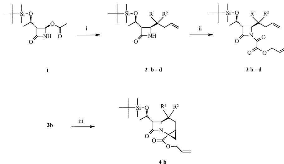
Scheme 2. Reagents: (i) (b) 2-allylmaleic acid diethyl ester or (c) 2-acetyl-pent-4-enoic acid ethyl ester or (d) 3-allylpentane-2,4-dione, NaH, THF (0°C→rt/2 h); (ii) allyl chloro-oxalate, Et 3 N, CH 2 Cl 2 (–20°C/1 h); (iii) P(OEt) 3 , xylene (reflux/9 h).
