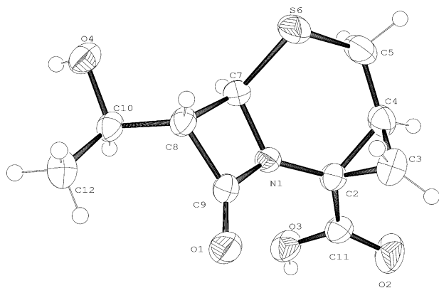
Figure 3. X-ray crystal structure of compound 6a.
