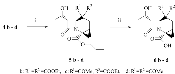
Scheme 4. Reagents: (i) (i\text{-Pr})_2\text{EtN}\cdot 3\text{HF} , anisole (50 °C/10 h); (ii) \text{Pd}(\text{PPh}_3)_4 , \text{PPh}_3 , sodium 2-ethyl hexanoate, \text{AcOEt} , (rt/3 h) \text{H}_2\text{O} , \text{H}_3\text{PO}_4 .
