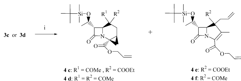
Scheme 3. Reagents: (i) \text{P}(\text{OEt})_3 , xylene (reflux/9 h).
